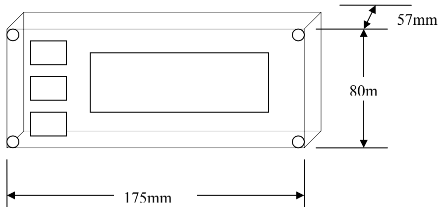
Front 4mm fixing screws 163mm X 68mm
